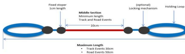
Figure 3 – Tether features
